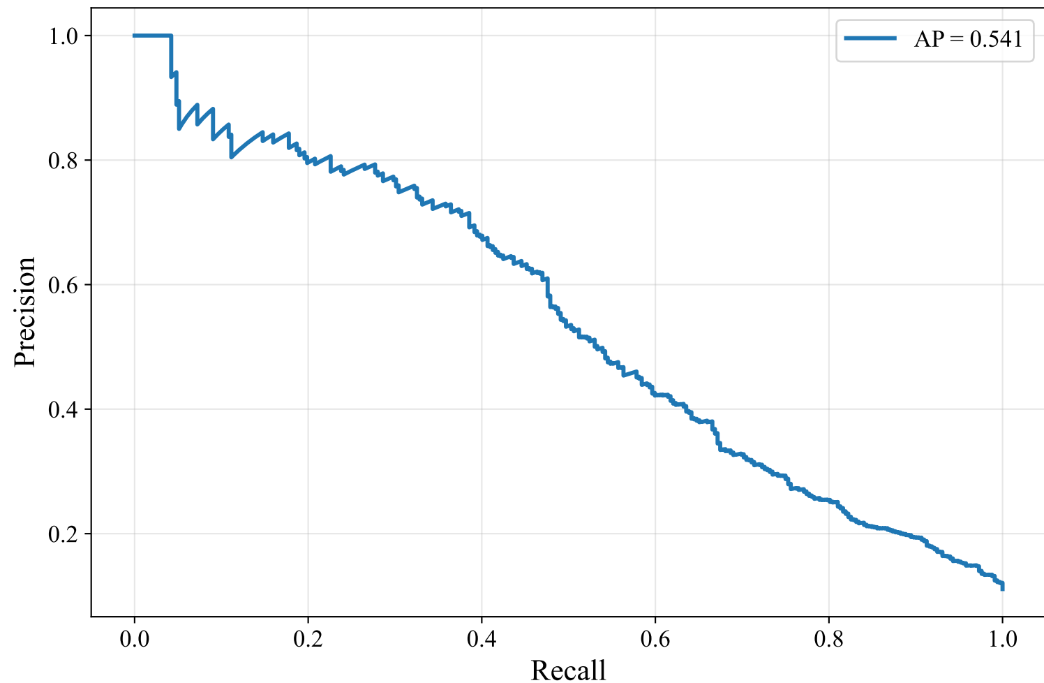
Precision-Recall Curve — GERMAN_MANUAL (intfloat/multilingual-e5-large-instruct, Random_Forest)
