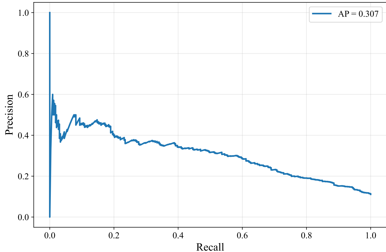
Precision-Recall Curve — GERMAN_MANUAL (intfloat/multilingual-e5-large-instruct, SVM)
