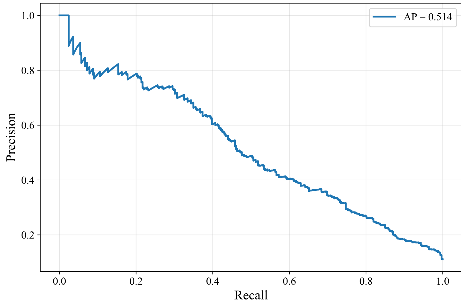
Precision-Recall Curve — GERMAN_MANUAL (snowflake-arctic-embed-l-v2.0, XGBoost)
