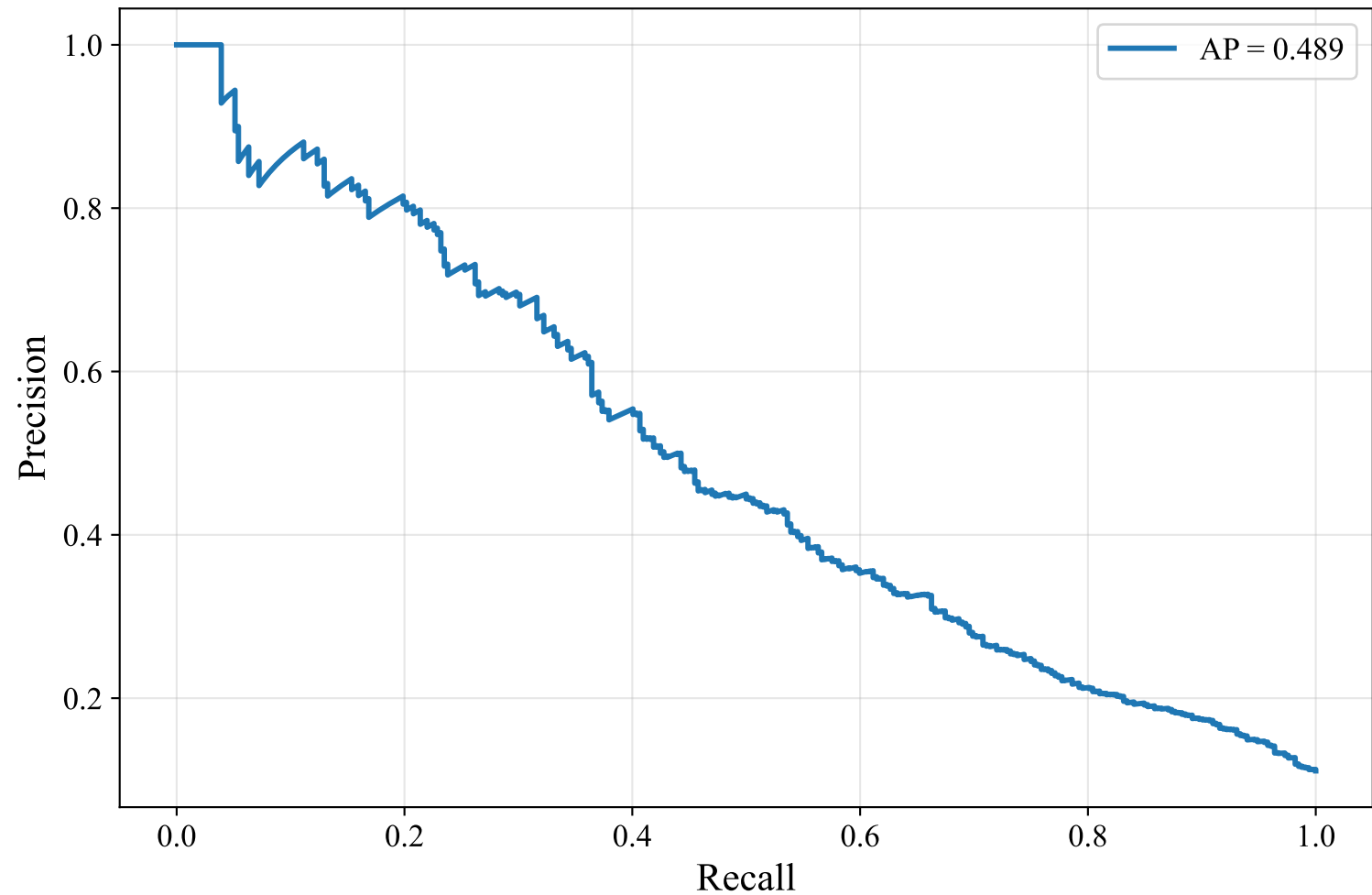
Precision-Recall Curve — GERMAN_MANUAL (upskyy/bge-m3-korean, LightGBM)
