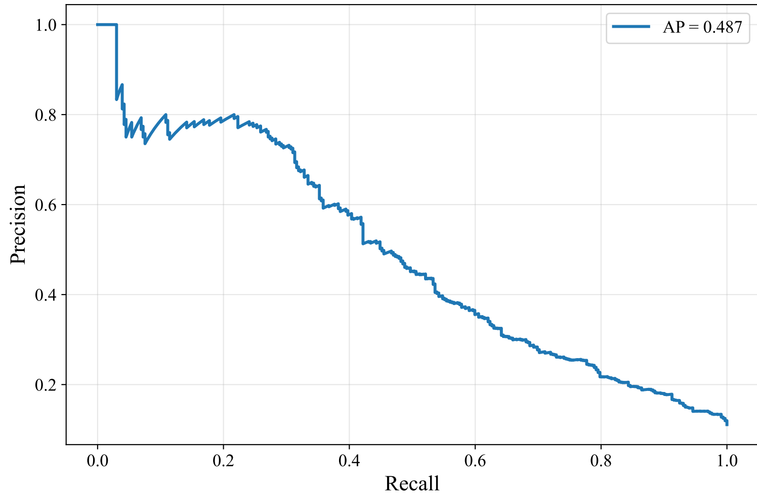
Precision-Recall Curve — GERMAN_MANUAL (upskyy/bge-m3-korean, Random_Forest)
