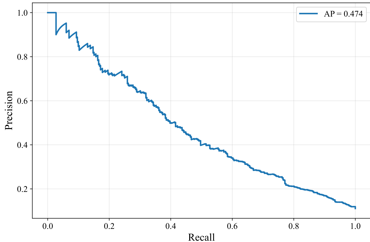
Precision-Recall Curve — GERMAN_MANUAL (xlm-roberta-base, XGBoost)
