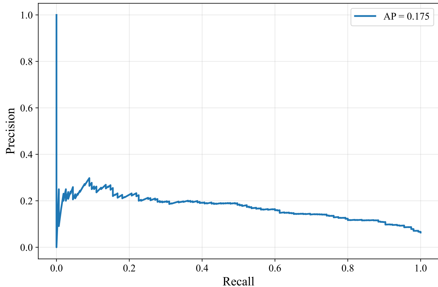
Precision-Recall Curve — SWEDEN_MANUAL (bert-base-multilingual-uncased, Random_Forest)
