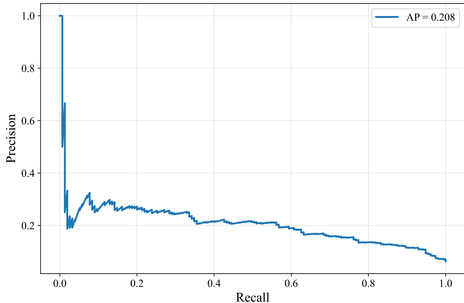
Precision-Recall Curve — SWEDISH_MANUAL (intfloat/multilingual-e5-large-instruct, LightGBM)
