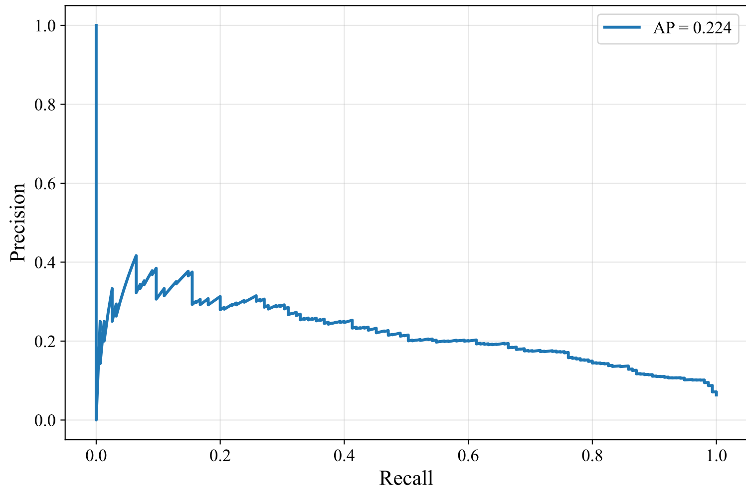
Precision-Recall Curve — SWEDISH_MANUAL (intfloat/multilingual-e5-large-instruct, Random_Forest)
