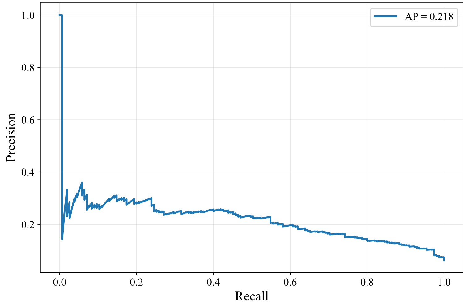
Precision-Recall Curve — SWEDISH_MANUAL (intfloat/multilingual-e5-large-instruct, XGBoost)
