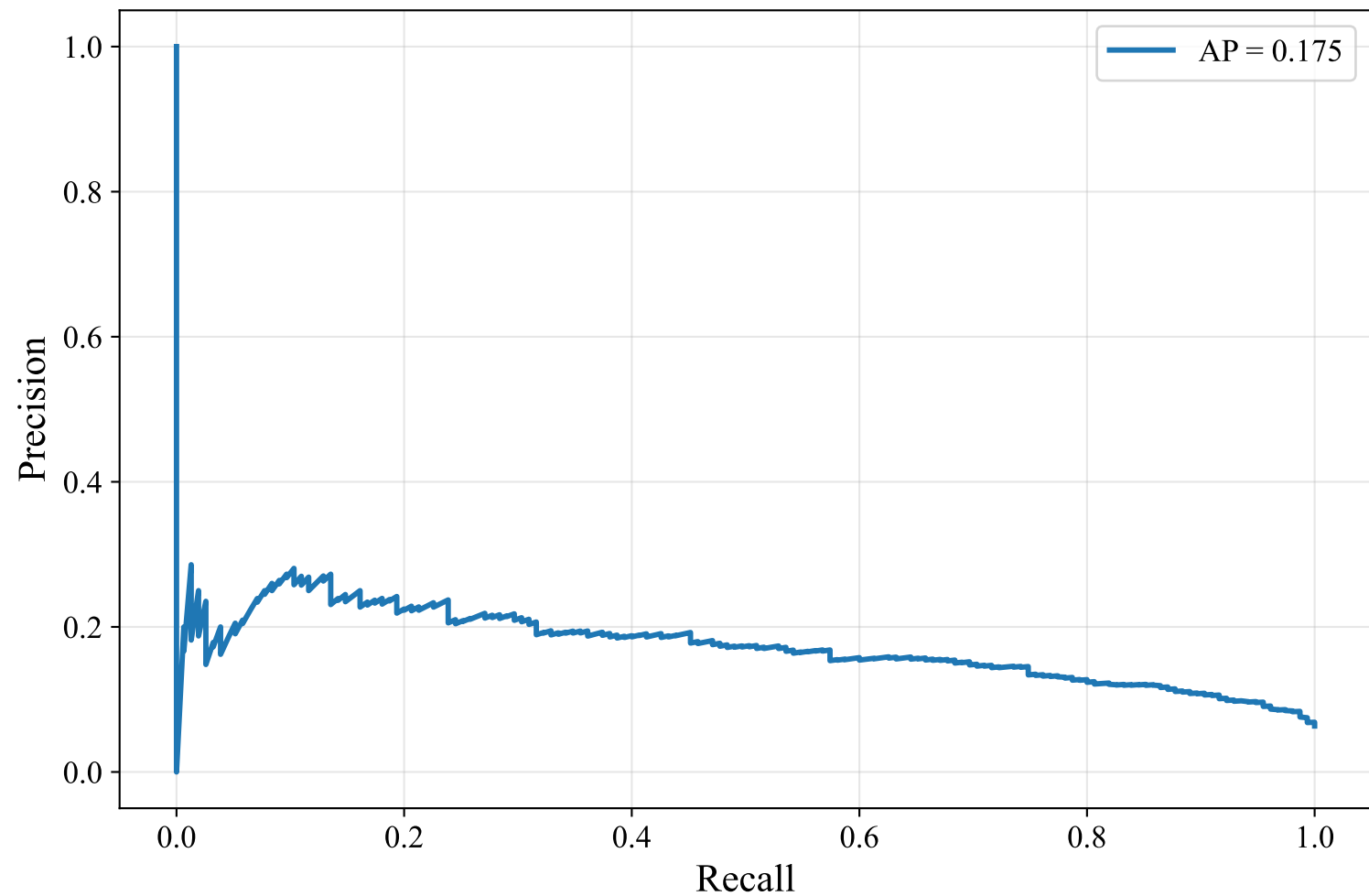
Precision-Recall Curve — SWEDISH_MANUAL (paraphrase-multilingual-mpnet-base-v2, Random_Forest)
