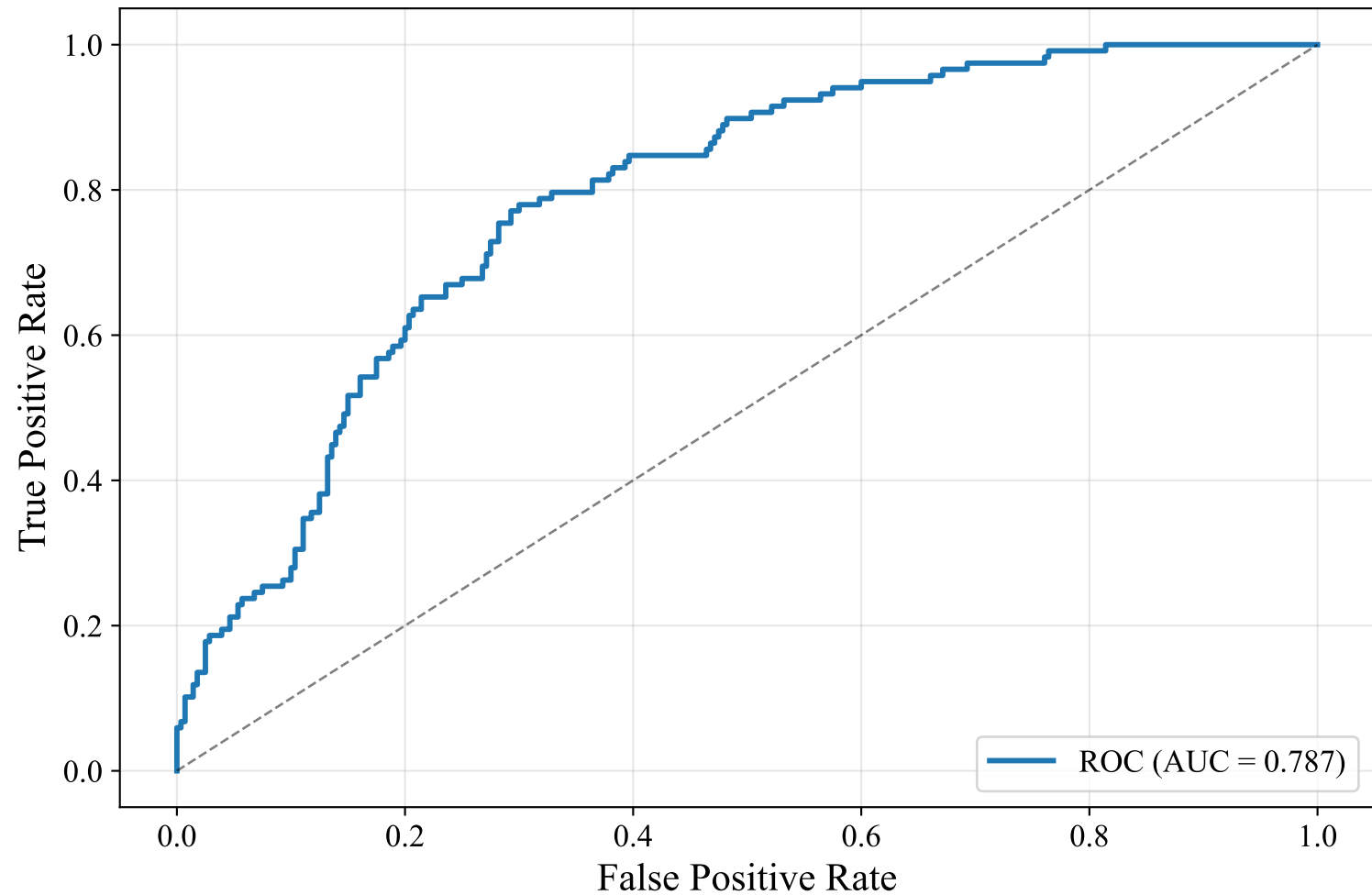
ROC Curve — DUTCH_MANUAL (bert-base-multilingual-uncased, XGBoost)
