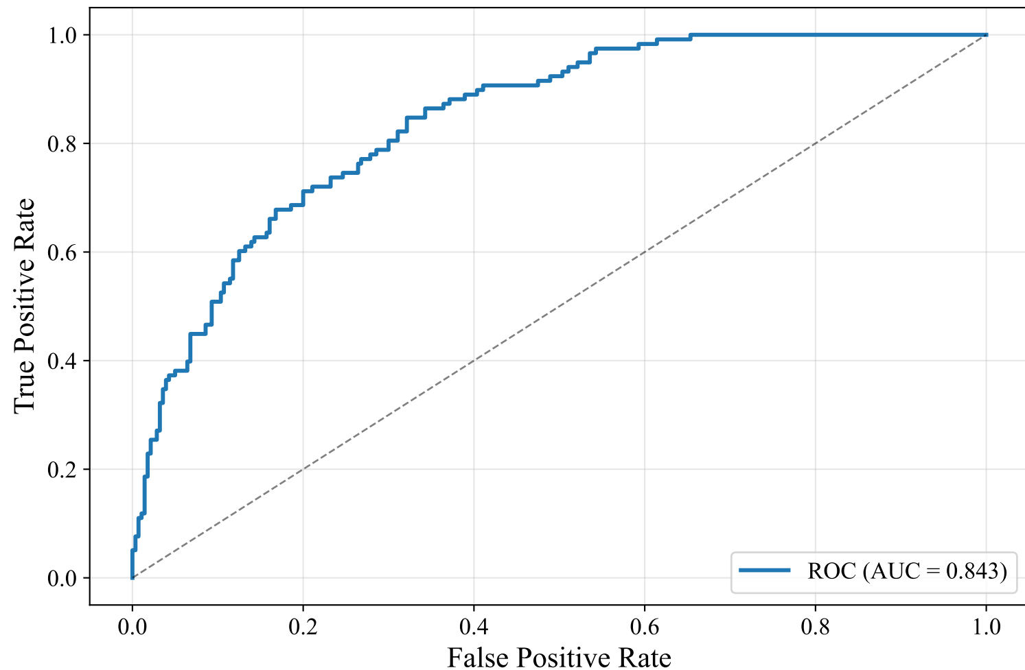
ROC Curve — DUTCH_MANUAL (intfloat/multilingual-e5-large-instruct, LightGBM)
