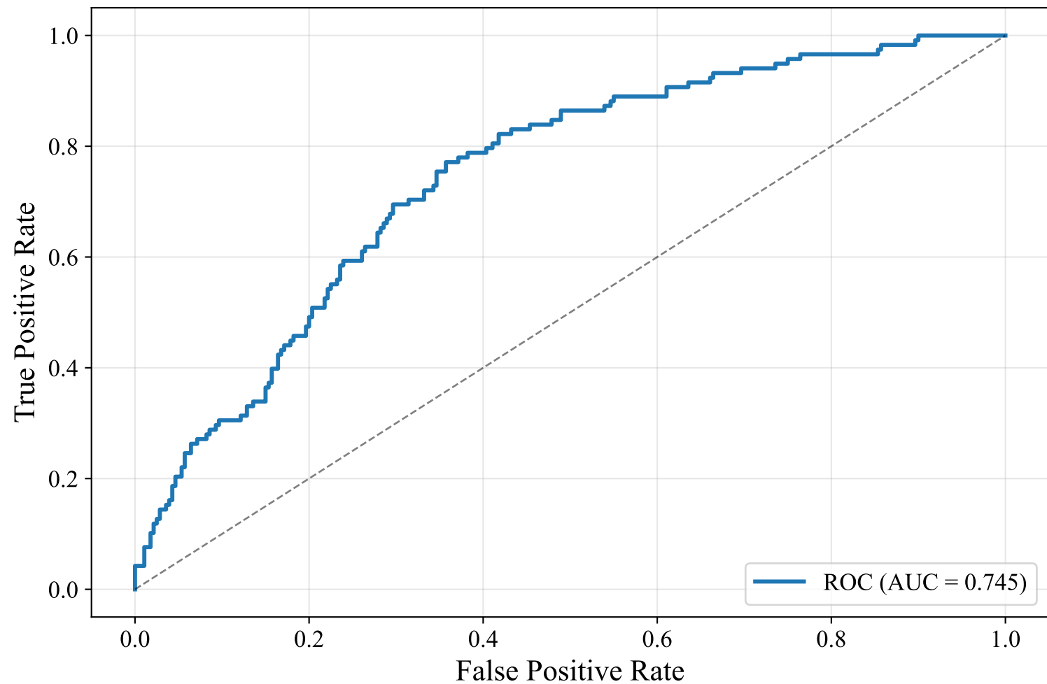
ROC Curve — DUTCH_MANUAL (intfloat/multilingual-e5-large-instruct, SVM)
