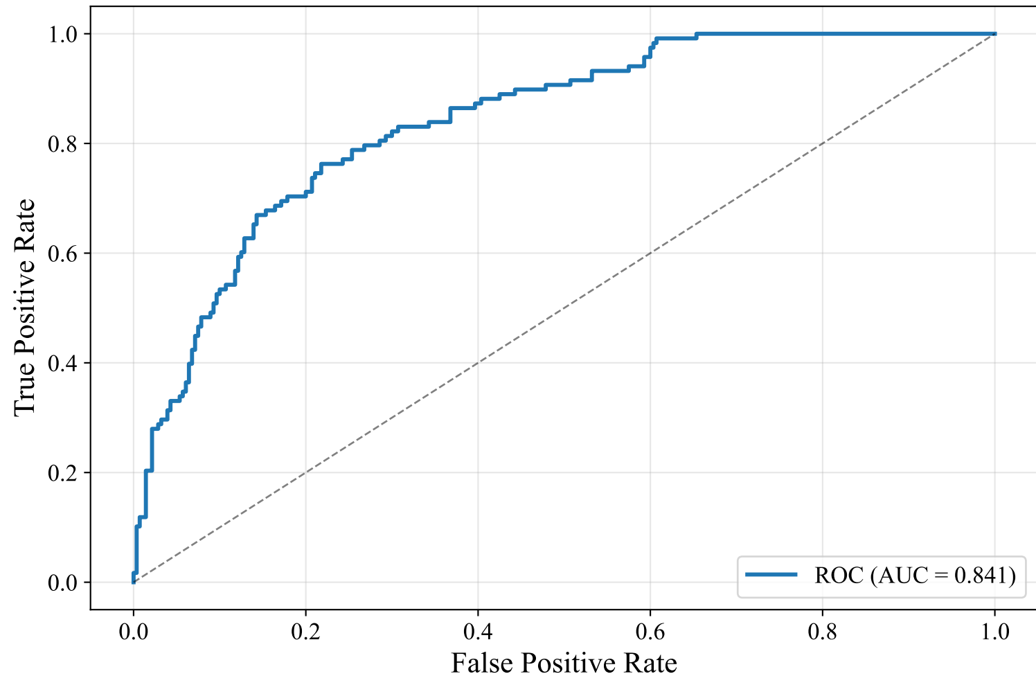
ROC Curve — DUTCH_MANUAL (intfloat/multilingual-e5-large-instruct, XGBoost)
