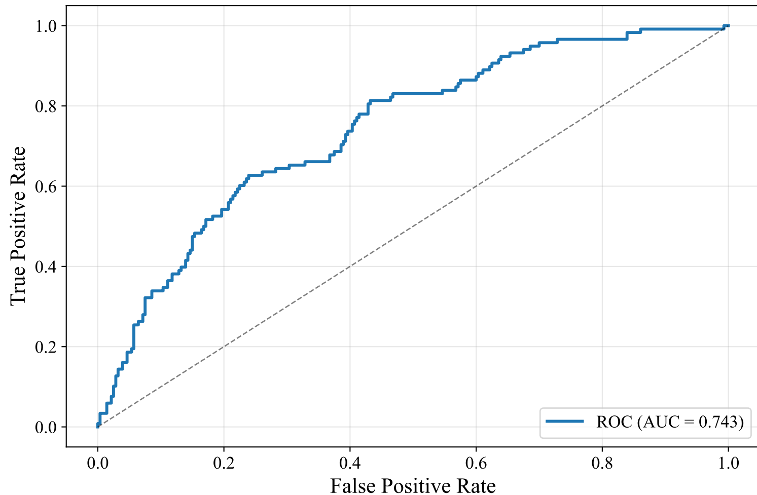
ROC Curve — DUTCH MANUAL (paraphrase-multilingual-MiniLM-L12-v2, SVM)
