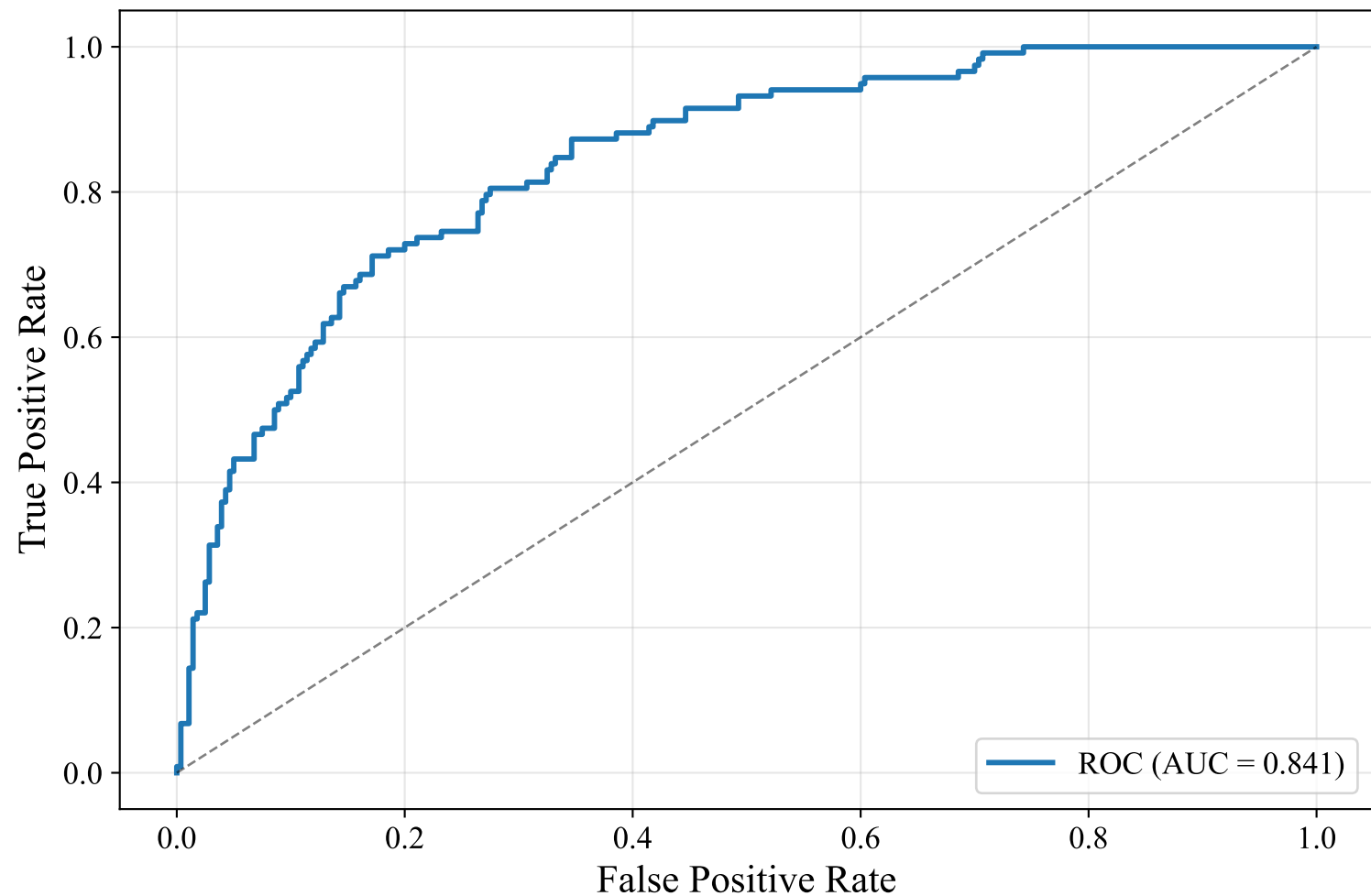
ROC Curve — DUTCH_MANUAL (snowflake-arctic-embed-l-v2.0, XGBoost)
