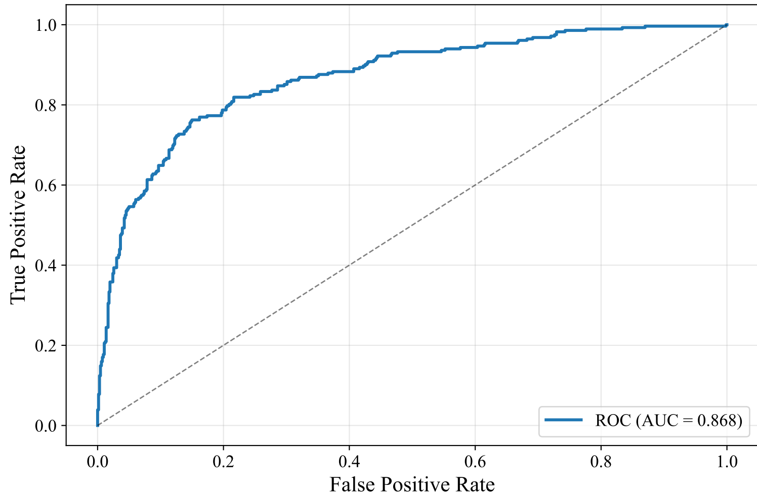
ROC Curve — ENGLISH_MANUAL (intfloat/multilingual-e5-large-instruct, XGBoost)
