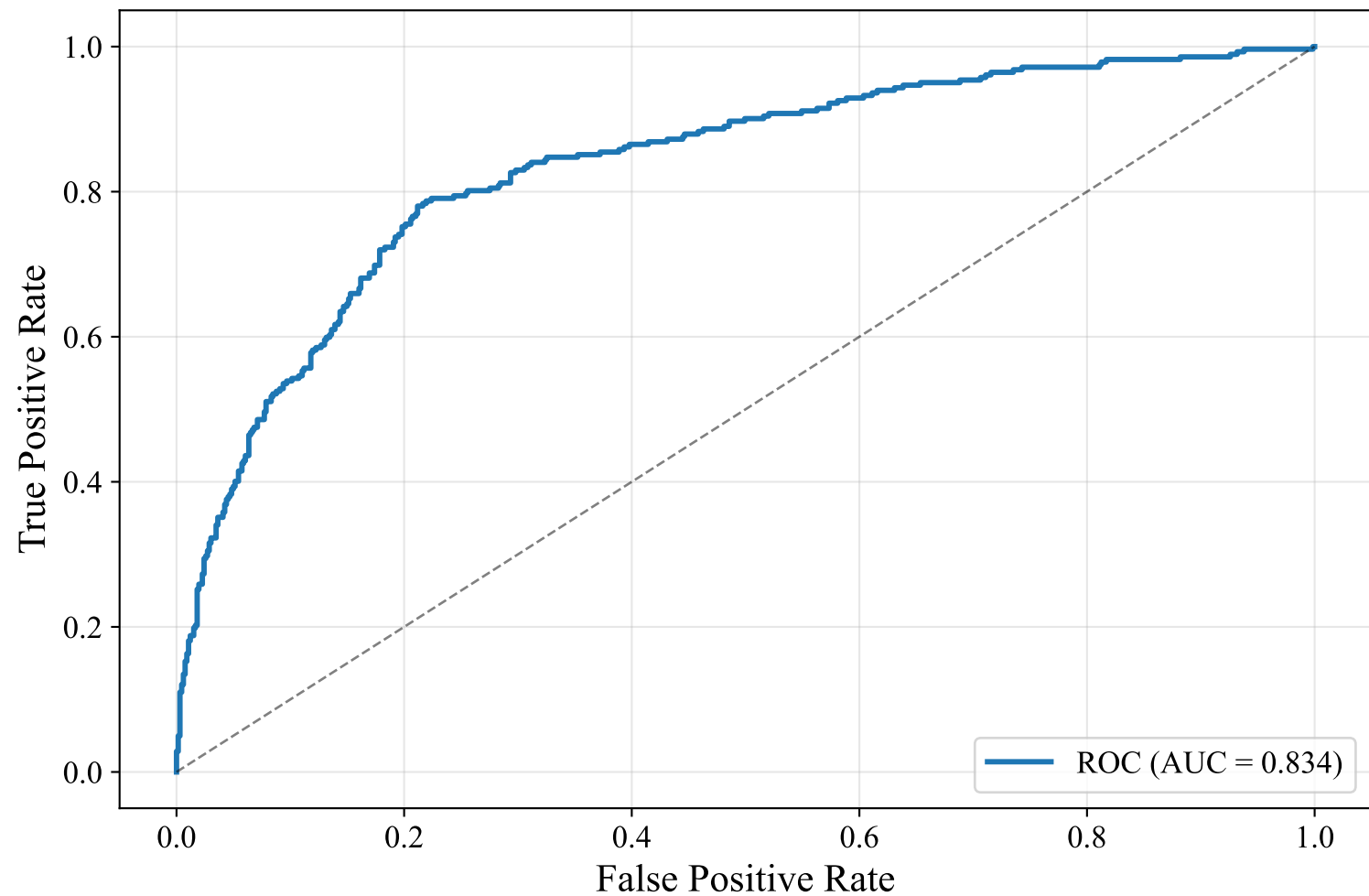
ROC Curve — ENGLISH_MANUAL (paraphrase-multilingual-mpnet-base-v2, SVM)
