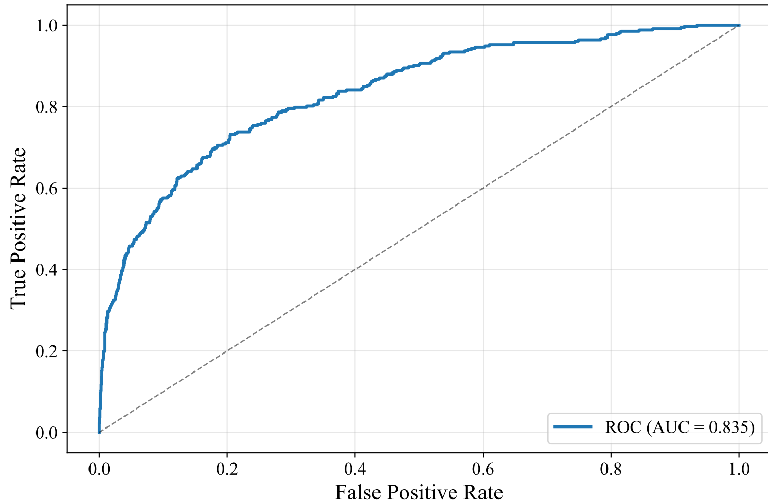
ROC Curve — GERMAN_MANUAL (snowflake-arctic-embed-l-v2.0, LightGBM)
