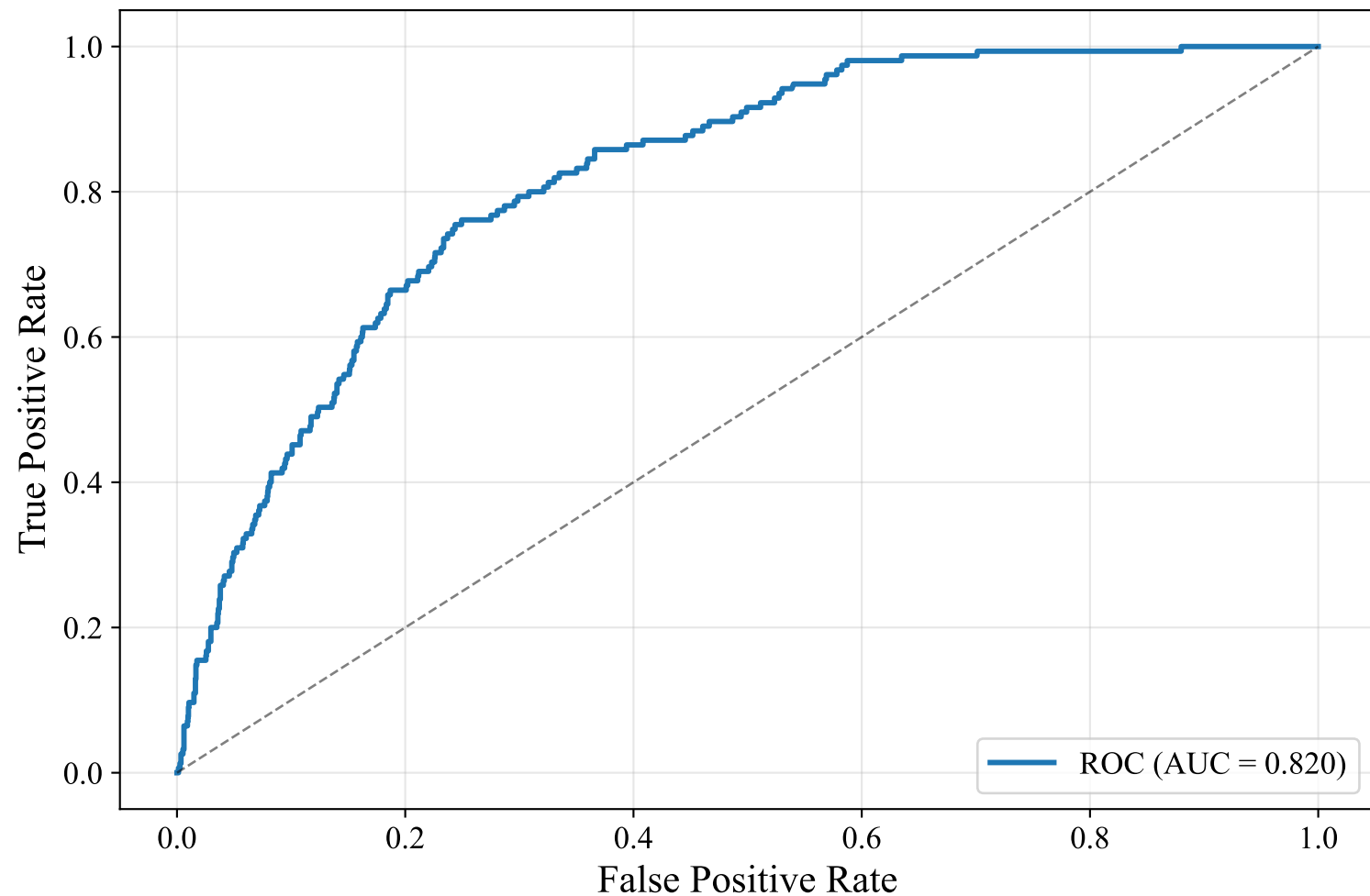
ROC Curve — SWEDISH_MANUAL (intfloat/multilingual-e5-large-instruct, Random_Forest)
