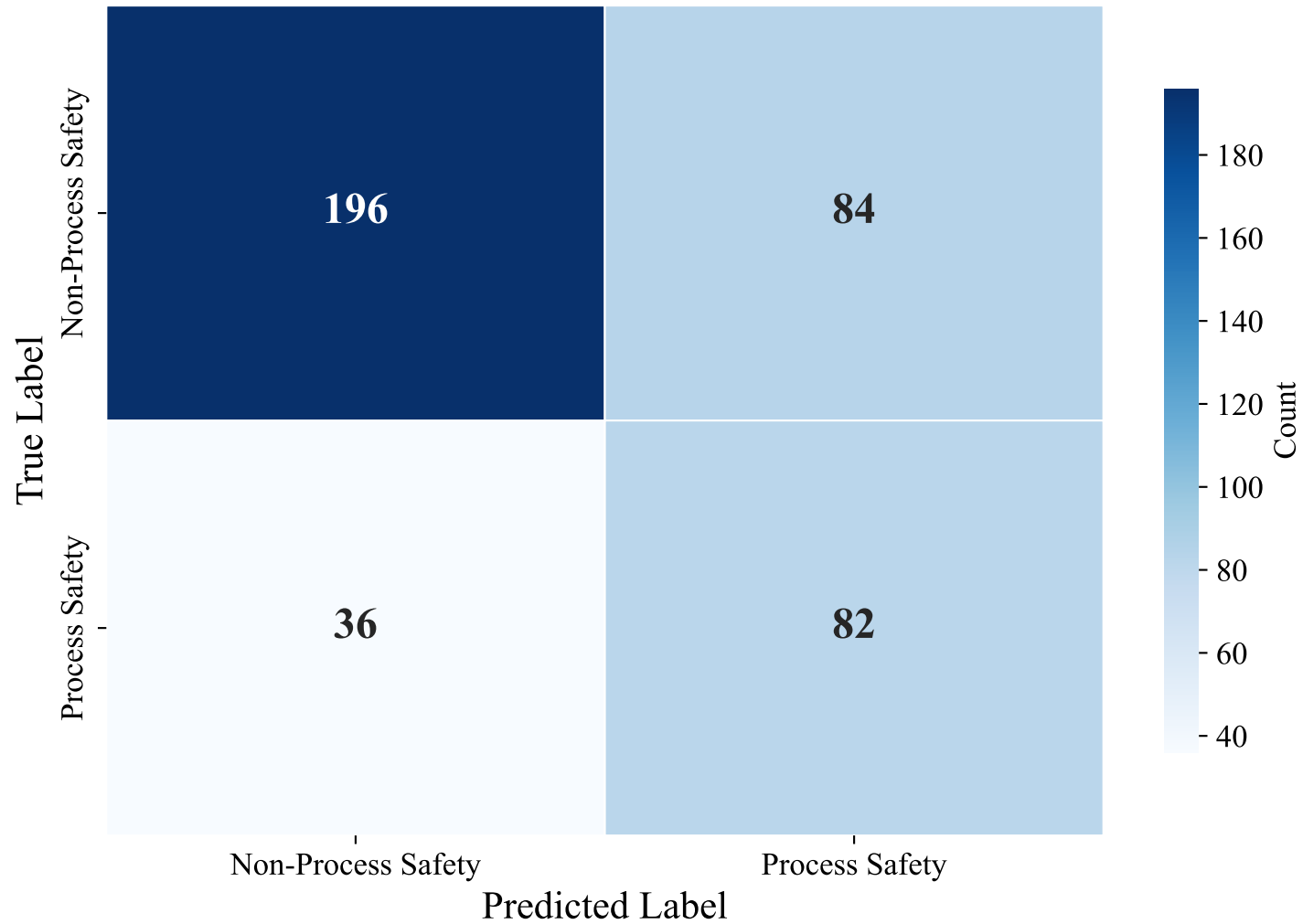
Confusion Matrix — DUTCH_MANUAL (bert-base-multilingual-uncased, LightGBM_Optimized)
