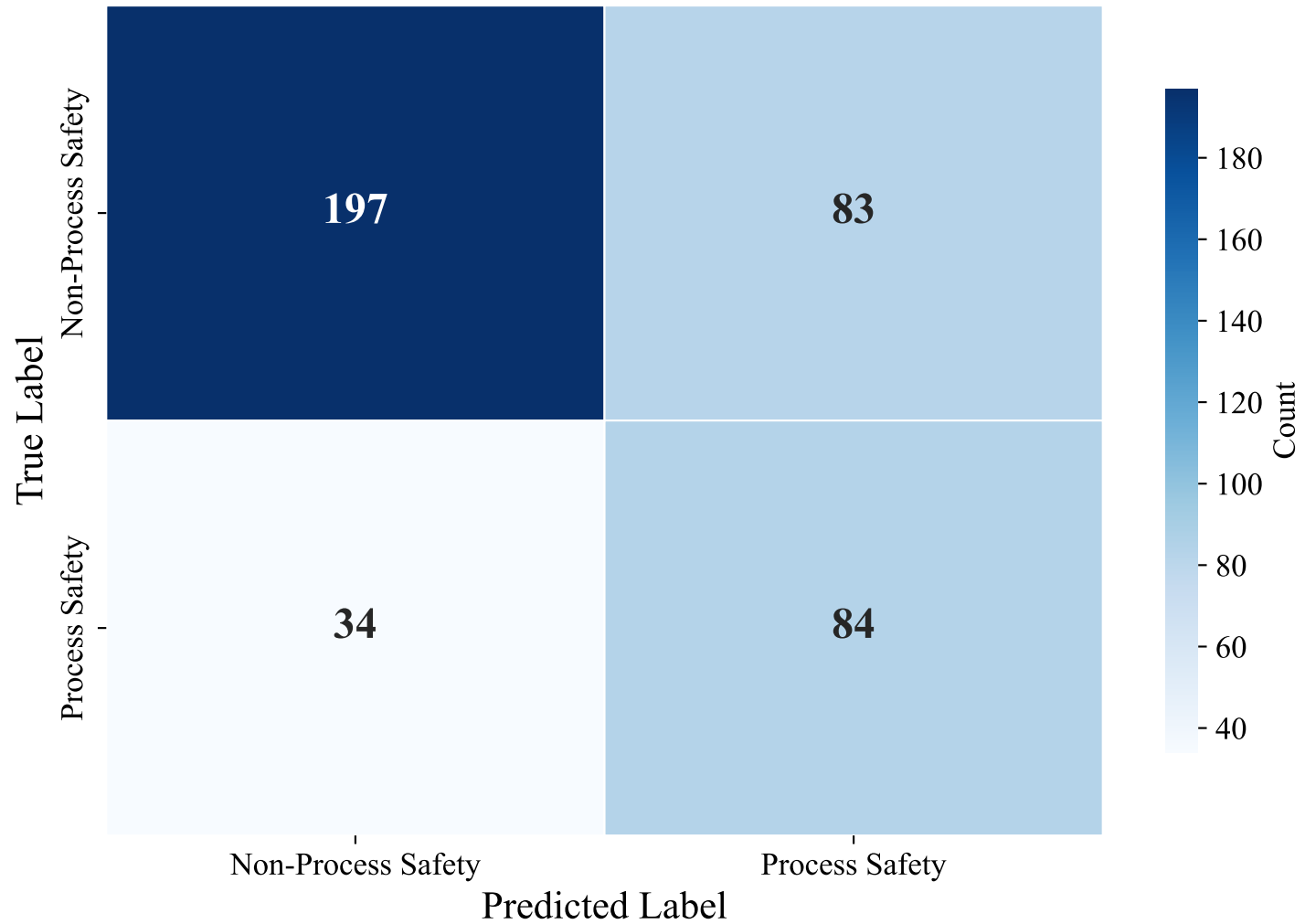
Confusion Matrix — DUTCH_MANUAL (bert-base-multilingual-uncased, XGBoost)
