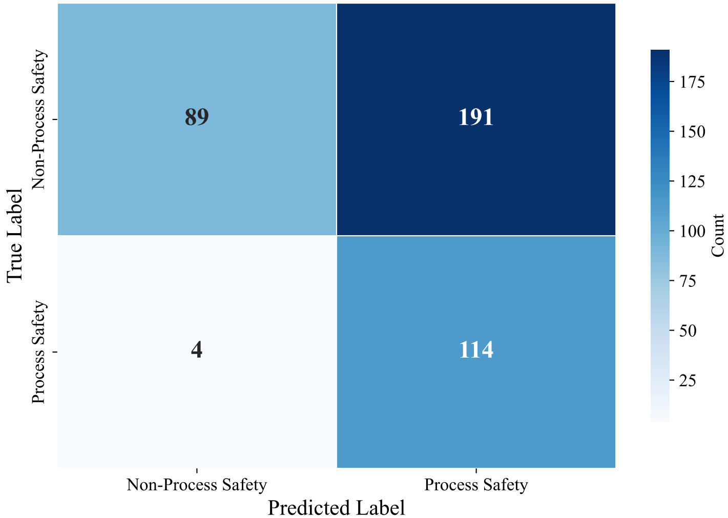
Confusion Matrix — DUTCH_MANUAL (efederici/e5-base-multilingual-4096, Random_Forest_Optimized)
