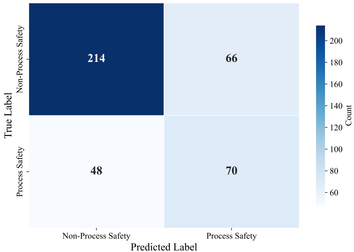
Confusion Matrix — DUTCH_MANUAL (efederici/e5-base-multilingual-4096, SVM)
