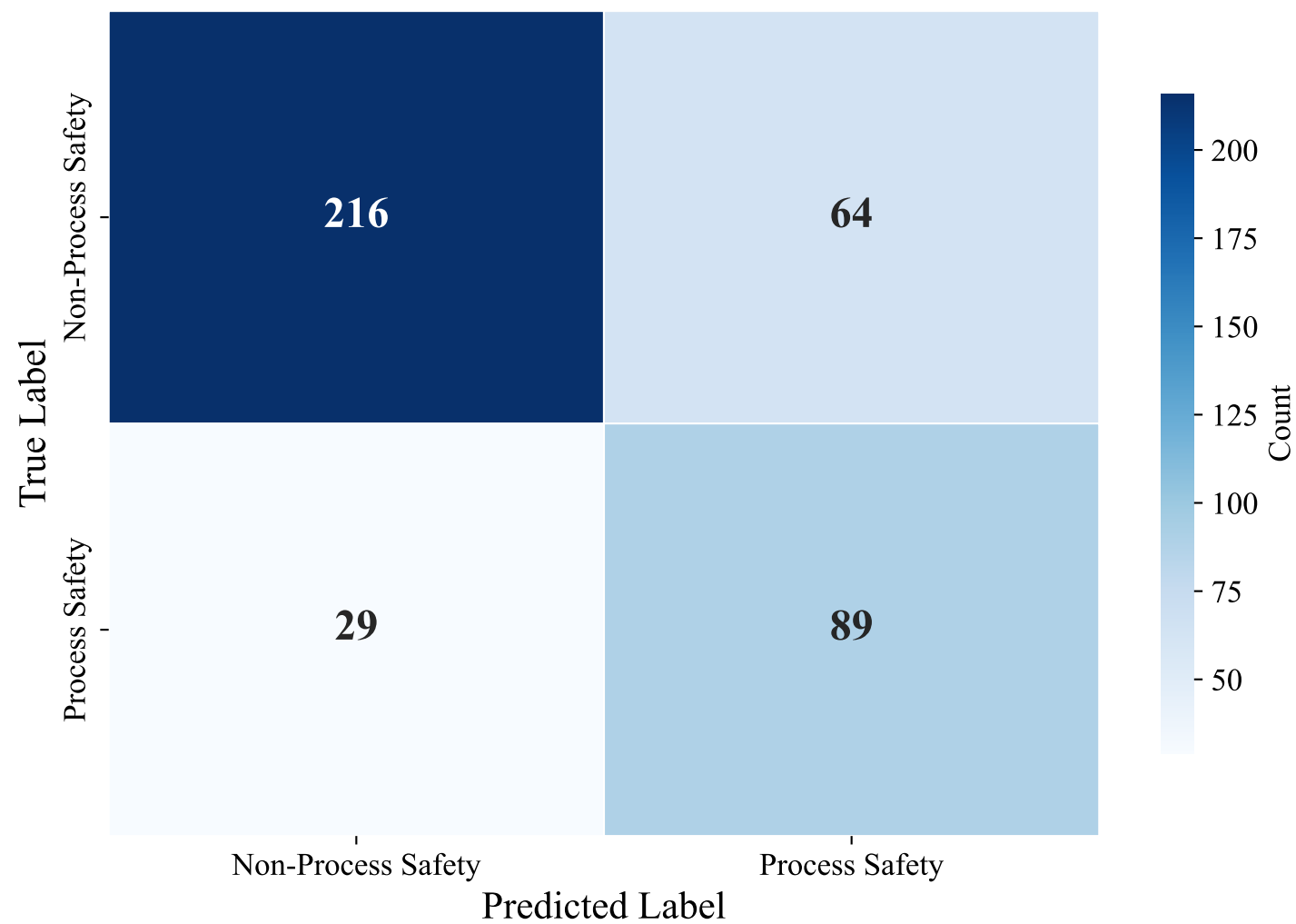
Confusion Matrix — DUTCH_MANUAL (intfloat/multilingual-e5-large-instruct, LightGBM)
