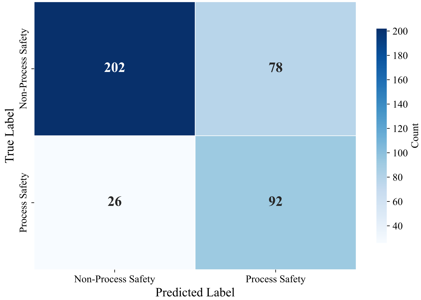
Confusion Matrix — DUTCH_MANUAL (intfloat/multilingual-e5-large-instruct, XGBoost)
