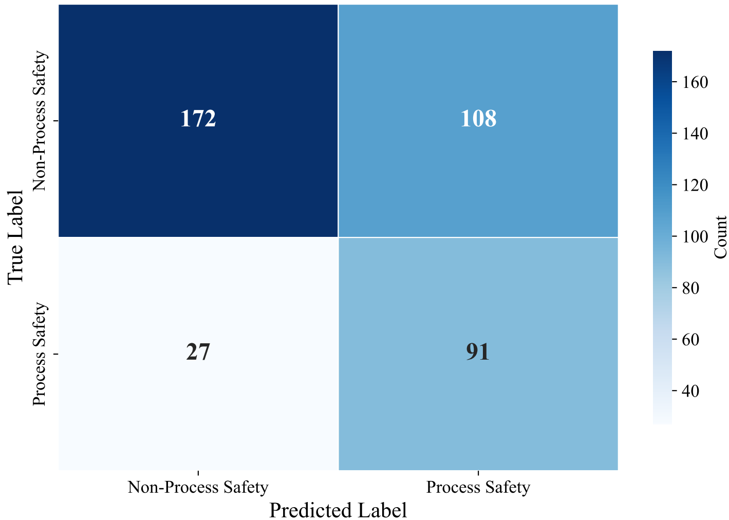
Confusion Matrix — DUTCH_MANUAL (paraphrase-multilingual-mpnet-base-v2, Random_Forest)
