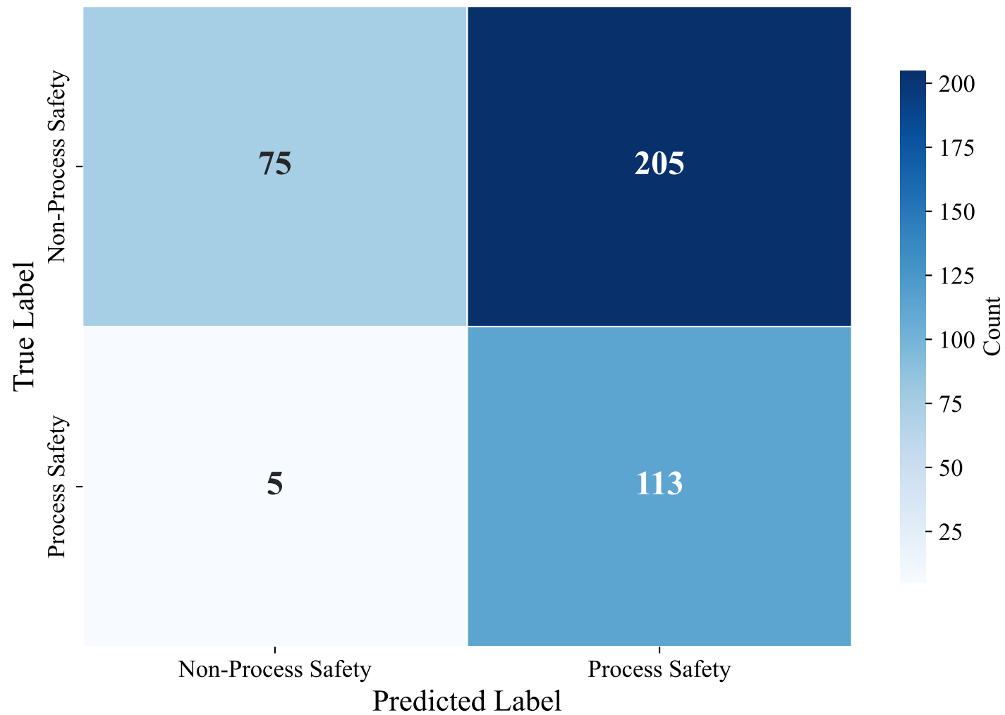
Confusion Matrix — DUTCH_MANUAL (paraphrase-multilingual-mpnet-base-v2, Random_Forest_Optimized)
