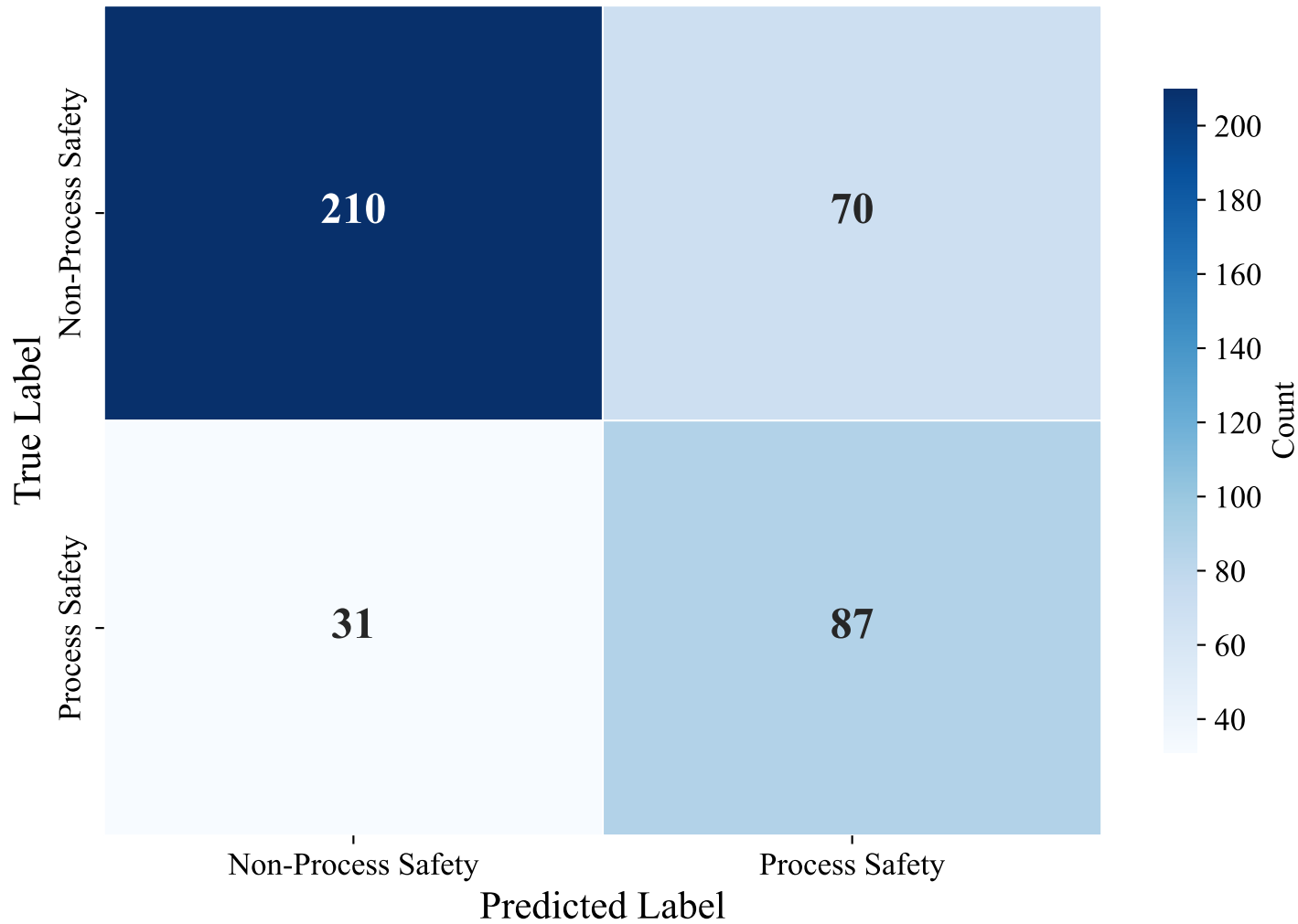
Confusion Matrix — DUTCH_MANUAL (snowflake-arctic-embed-l-v2.0, LightGBM_Optimized)
