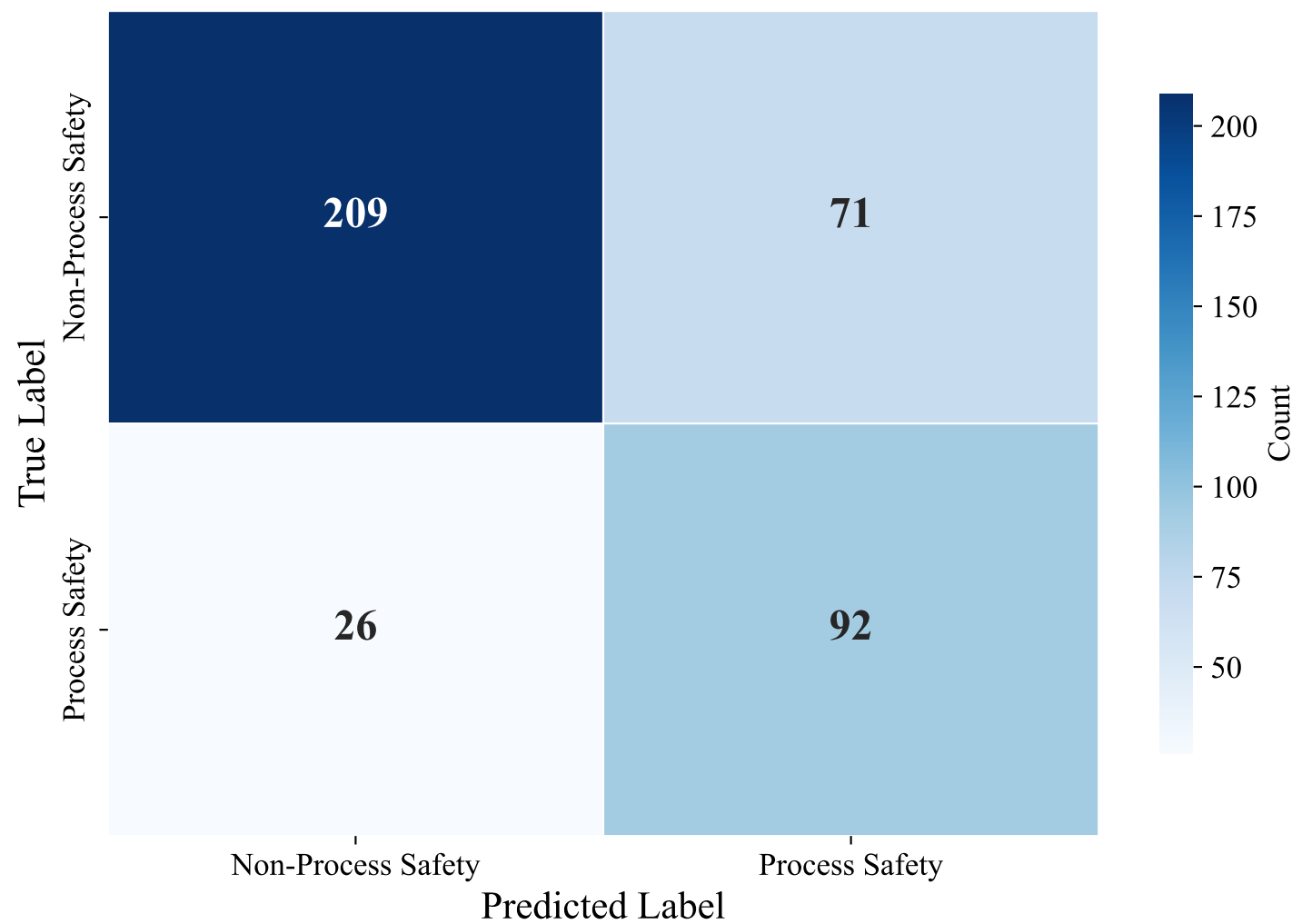
Confusion Matrix — DUTCH_MANUAL (upskyy/bge-m3-korean, LightGBM_Optimized)
