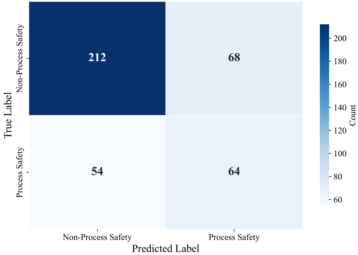
Confusion Matrix — DUTCH_MANUAL (upskyy/bge-m3-korean, SVM)
