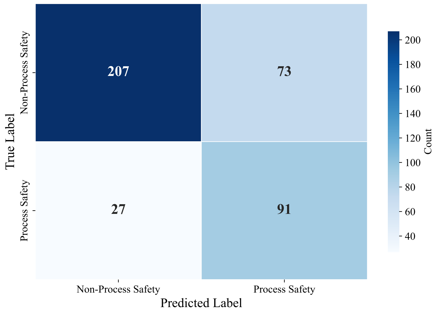
Confusion Matrix — DUTCH_MANUAL (upskyy/bge-m3-korean, Voting_Ensemble)
