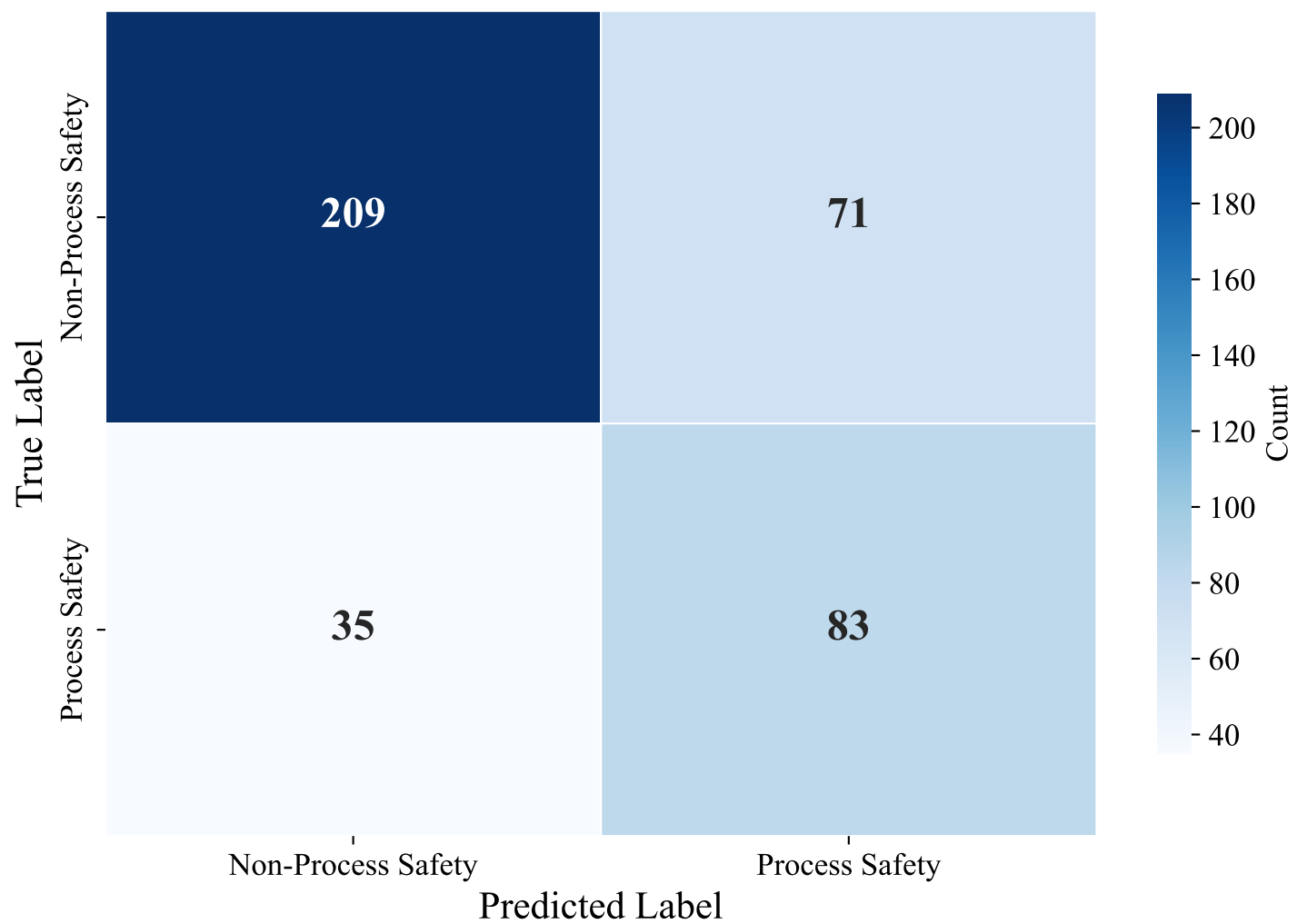
Confusion Matrix — DUTCH_MANUAL (xlm-roberta-base, LightGBM)
