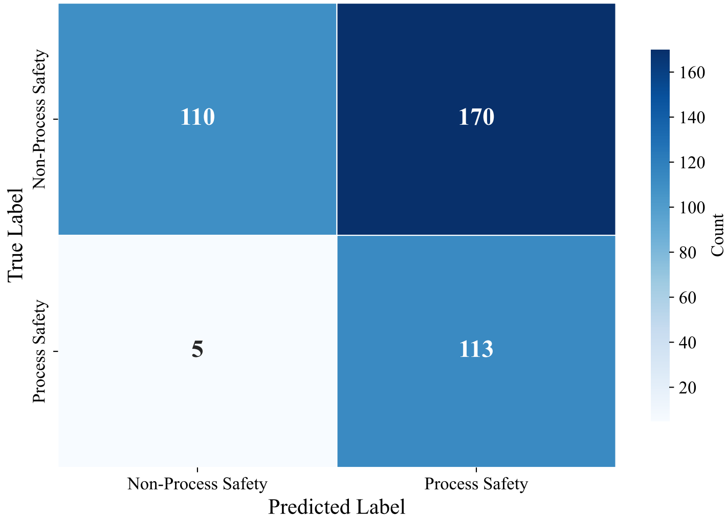
Confusion Matrix — DUTCH_MANUAL (xlm-roberta-base, Random_Forest_Optimized)
