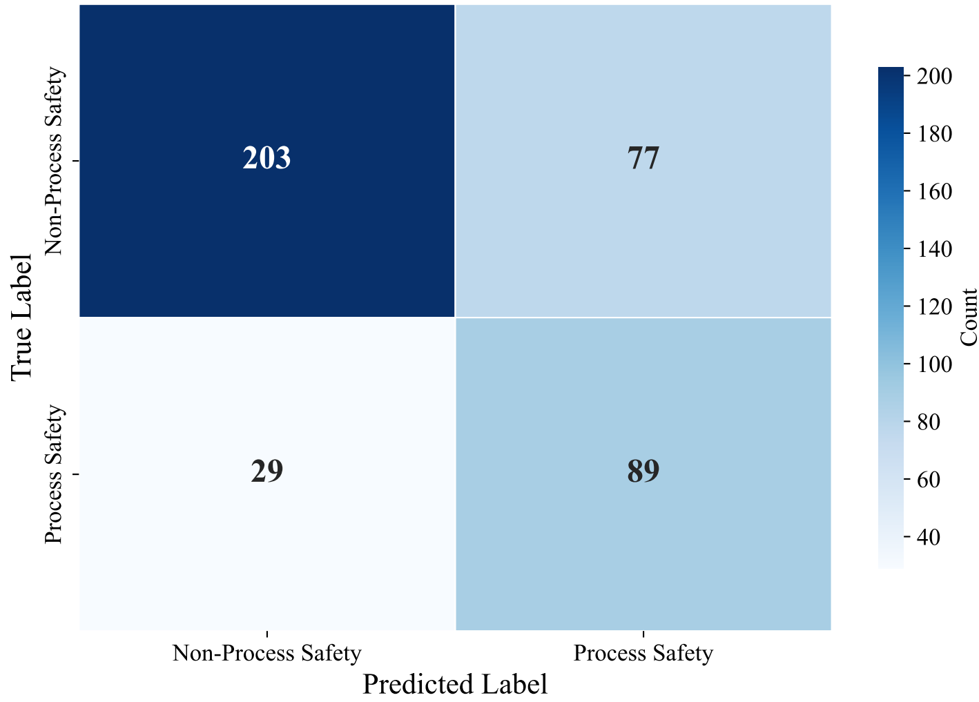
Confusion Matrix — DUTCH_MANUAL (xlm-roberta-base, Voting_Ensemble)
