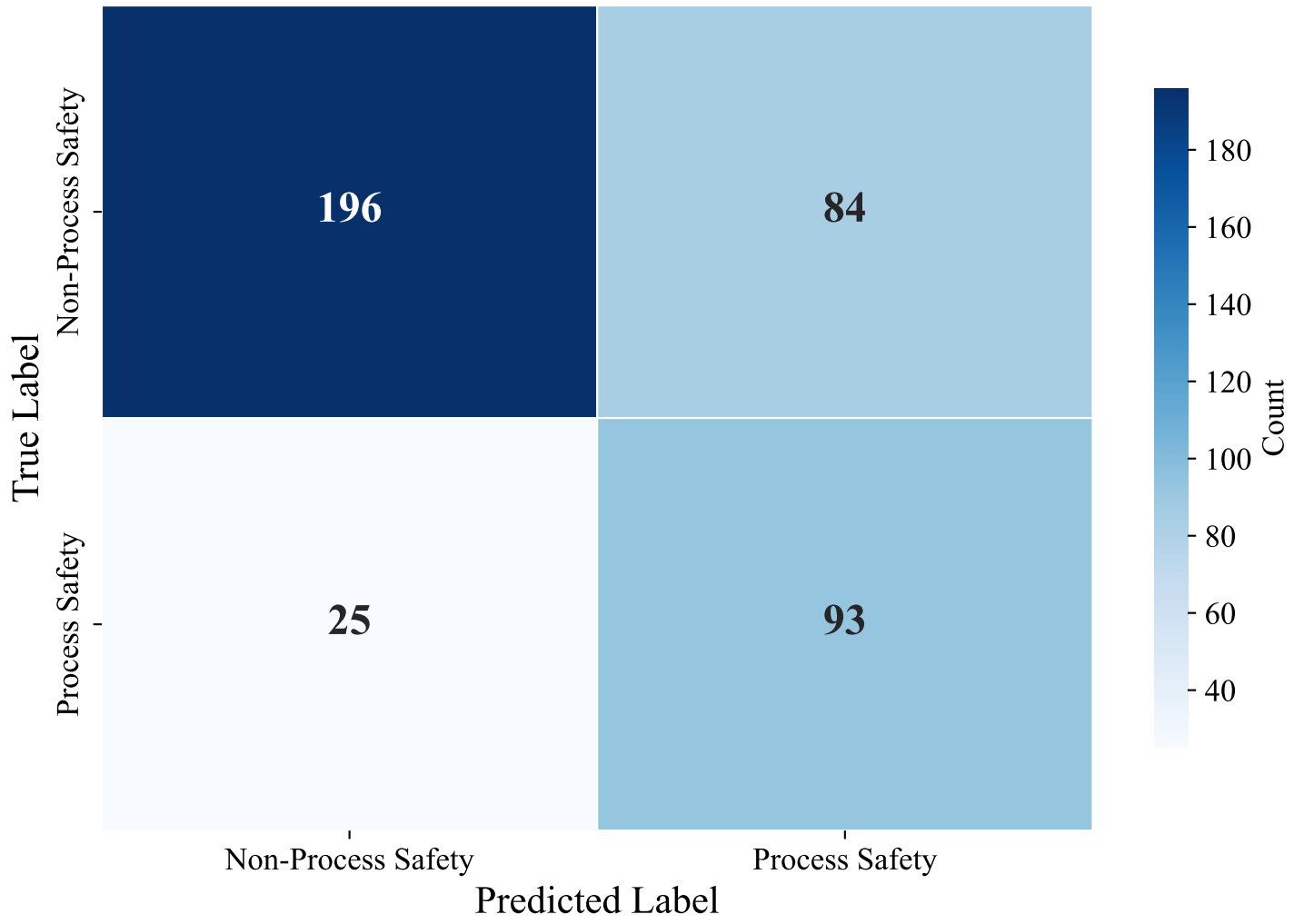
Confusion Matrix — DUTCH_MANUAL (xlm-roberta-base, XGBoost)
