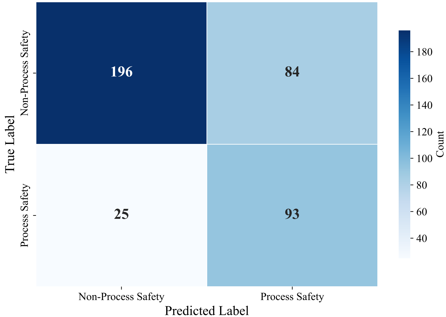
Confusion Matrix — DUTCH_MANUAL (xlm-roberta-base, XGBoost_Optimized)
