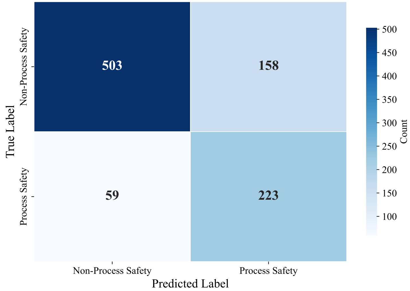
Confusion Matrix — ENGLISH_MANUAL (bert-base-multilingual-uncased, LightGBM)
