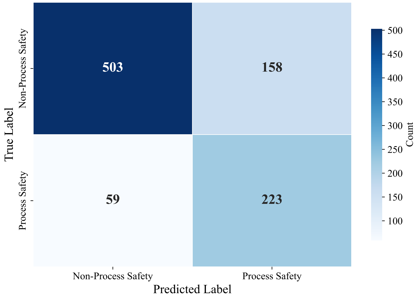
Confusion Matrix — ENGLISH_MANUAL (bert-base-multilingual-uncased, LightGBM_Optimized)
