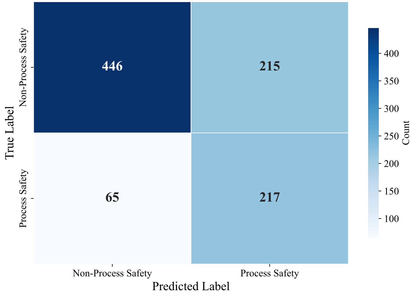
Confusion Matrix — ENGLISH_MANUAL (bert-base-multilingual-uncased, Random_Forest)
