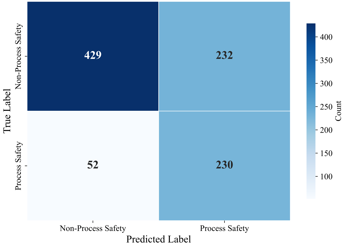
Confusion Matrix — ENGLISH_MANUAL (efederici/e5-base-multilingual-4096, Random_Forest)
