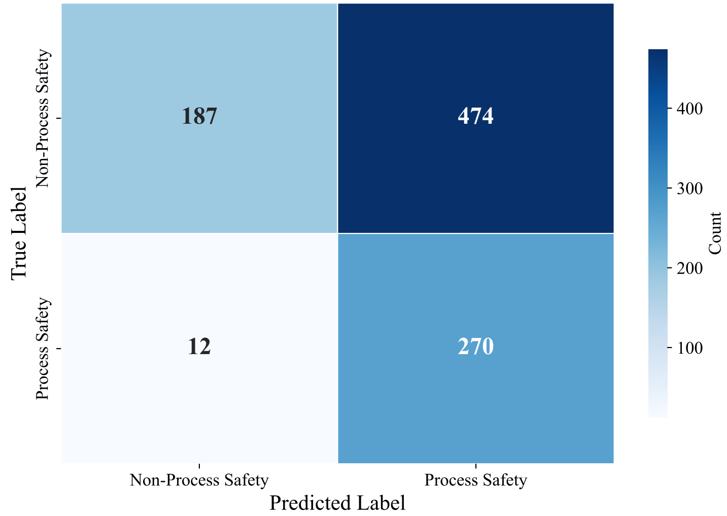
Confusion Matrix — ENGLISH_MANUAL (efederici/e5-base-multilingual-4096, Random_Forest_Optimized)
