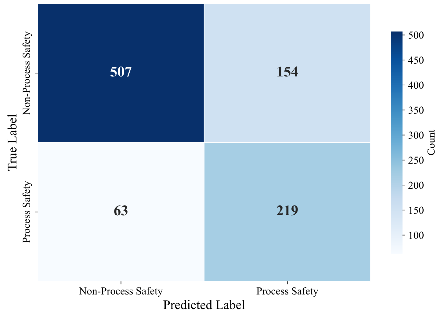
Confusion Matrix — ENGLISH_MANUAL (efederici/e5-base-multilingual-4096, XGBoost)
