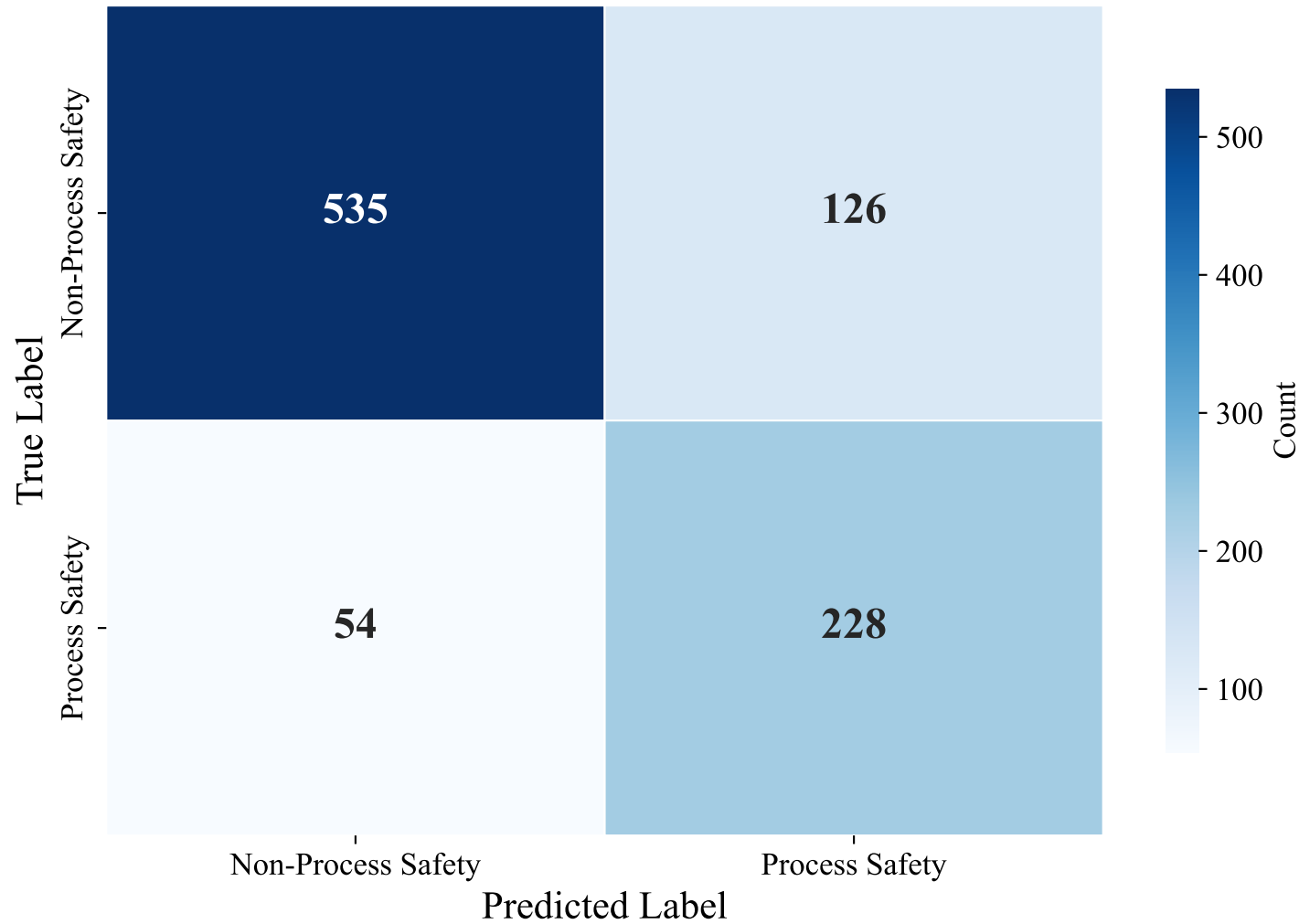
Confusion Matrix — ENGLISH_MANUAL (intfloat/multilingual-e5-large-instruct, LightGBM)
