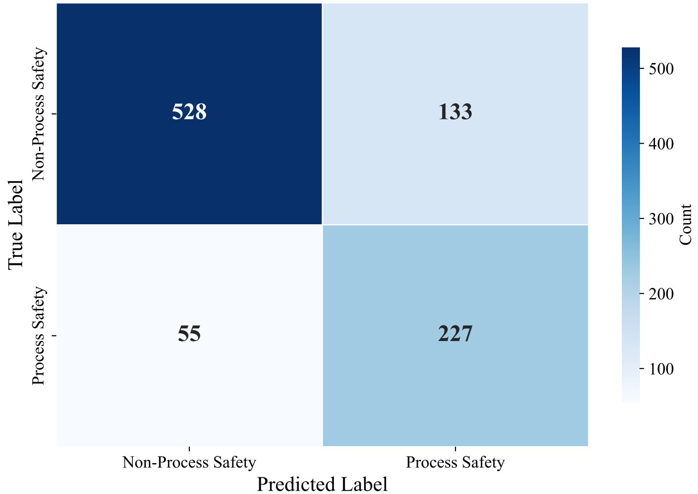
Confusion Matrix — ENGLISH_MANUAL (intfloat/multilingual-e5-large-instruct, XGBoost_Optimized)
