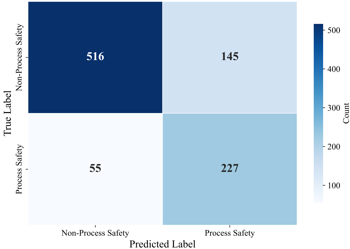
Confusion Matrix — ENGLISH_MANUAL (paraphrase-multilingual-MiniLM-L12-v2, XGBoost)
