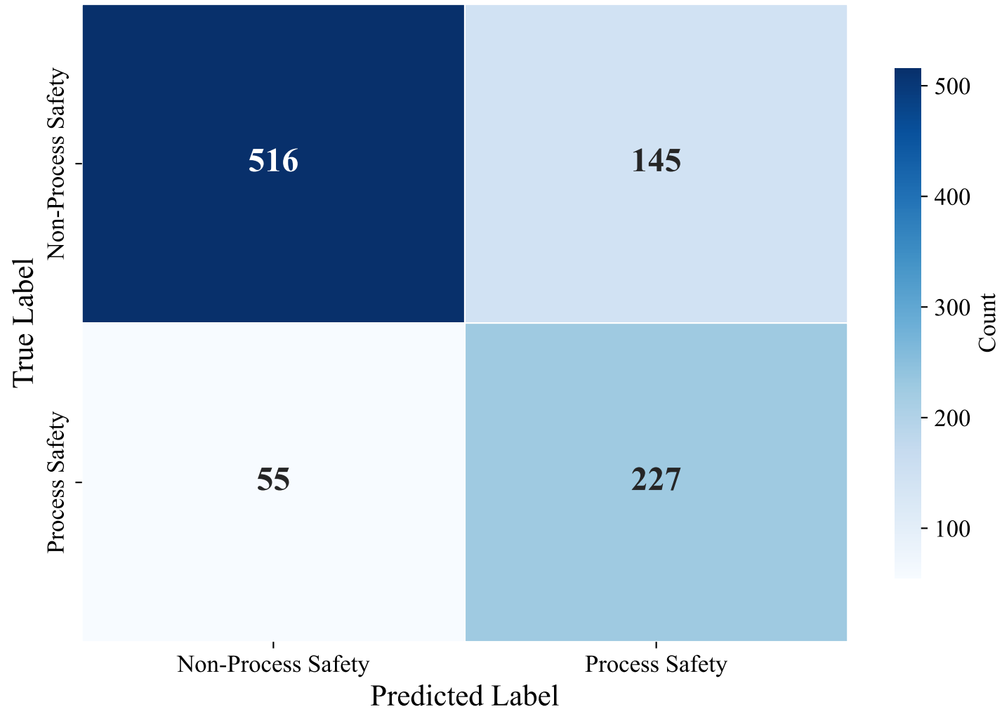
Confusion Matrix — ENGLISH_MANUAL (paraphrase-multilingual-MiniLM-L12-v2, XGBoost_Optimized)
