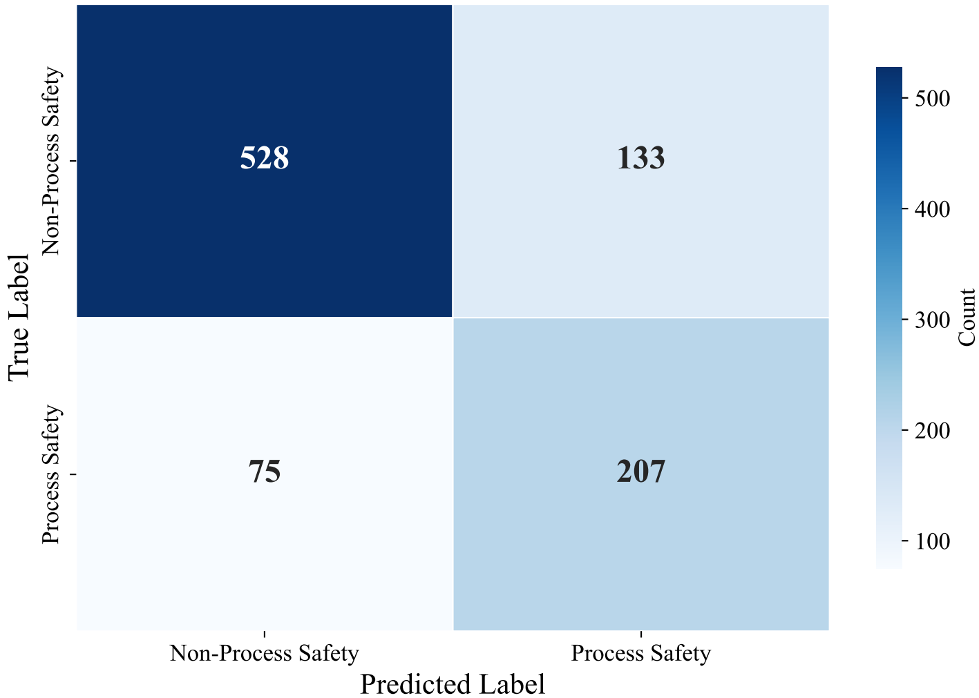
Confusion Matrix — ENGLISH_MANUAL (paraphrase-multilingual-mpnet-base-v2, SVM)
