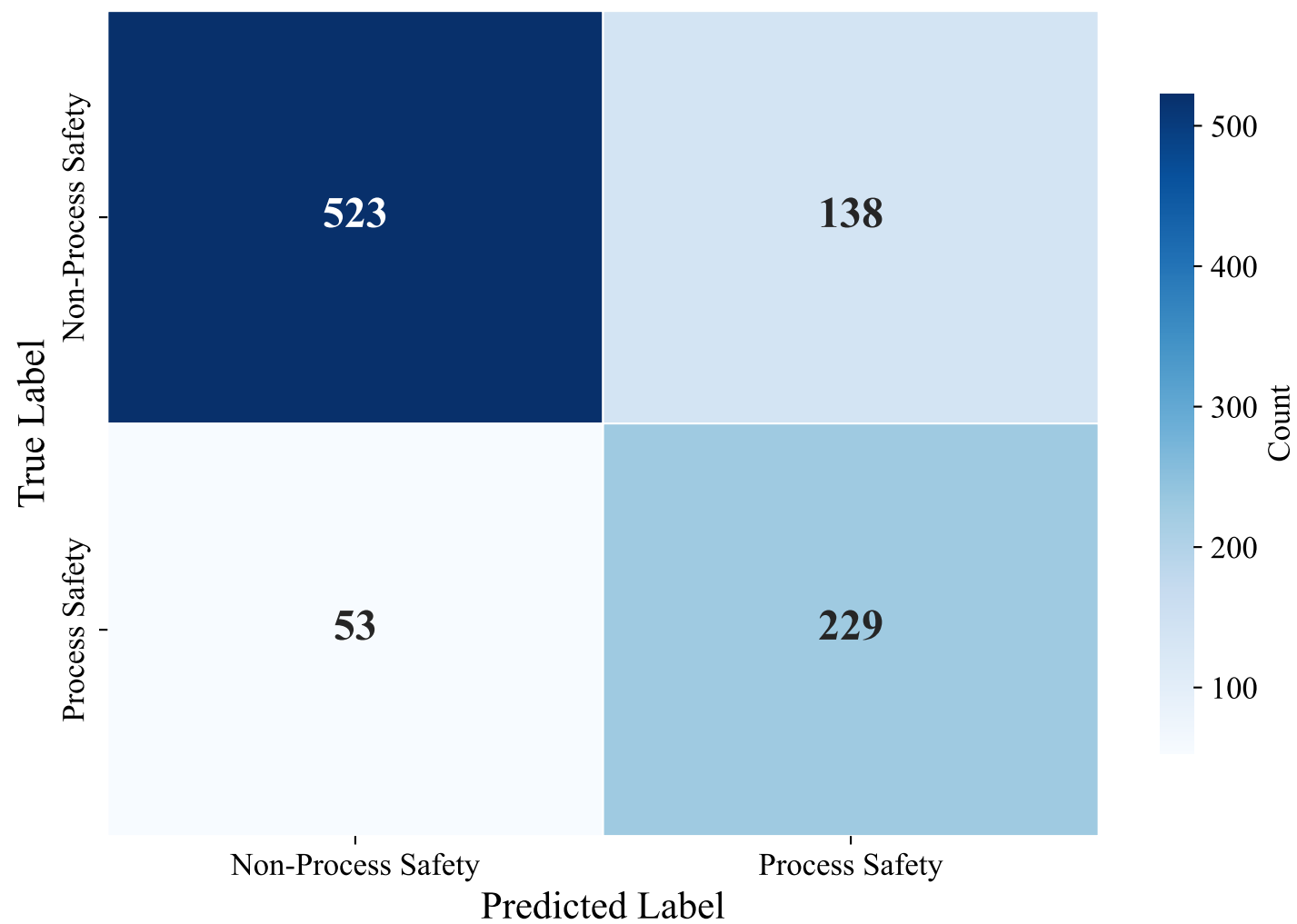
Confusion Matrix — ENGLISH_MANUAL (paraphrase-multilingual-mpnet-base-v2, XGBoost)
